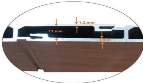
DETAIL OF DOUBLE WALL PANELED
